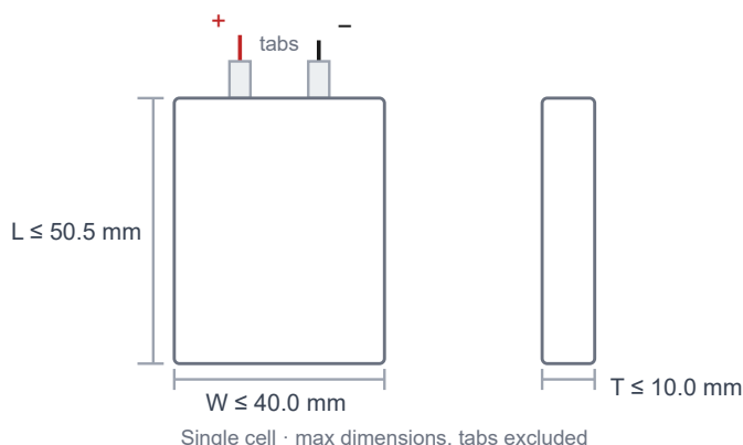
Cell drawing · single cell 104050 (not to scale)
