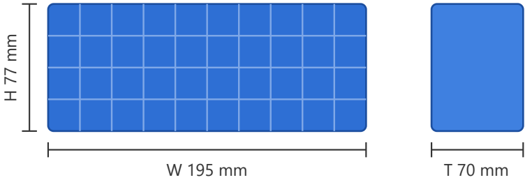
Pack dimensions (40 × 18650 cells, estimated) — not to scale
