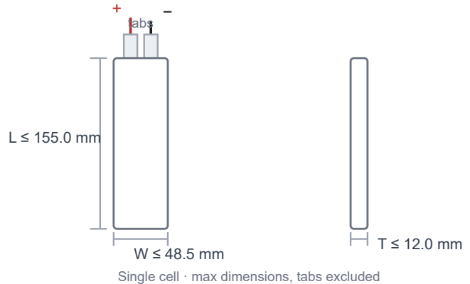
Cell drawing · single cell of pack 3849160 (not to scale)
