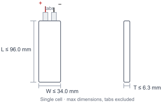
Cell drawing · single cell 633496 (not to scale)
