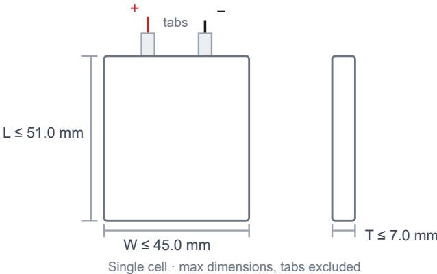
Cell drawing · single cell 704551 (not to scale)
