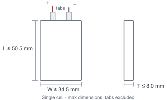
Cell drawing · single cell 803450 (not to scale)
